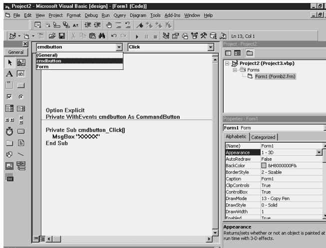
FIGURE 4.16 Once you've declared your control using WithEvents , you can see the control and its events in the drop-down lists of the Code window.
