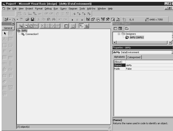
FIGURE 8.1▲ Adding the Data Environment Designer component to your project.
